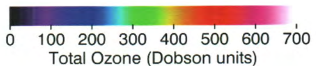
October Total Ozone 1979-2015
